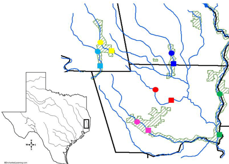
Figure 1. Sample location for the six river corridors sampled in the BITH. Colors correspond to sample localities in Fig. 2.
