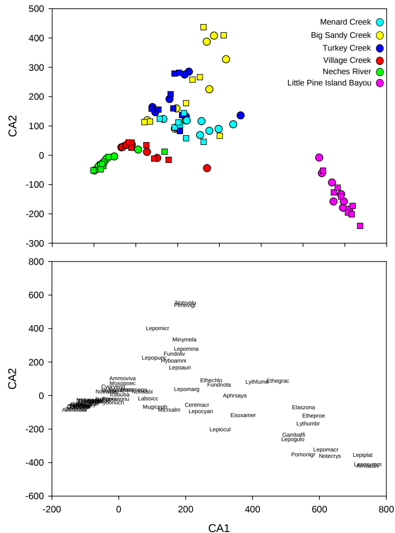
Figure 2. Ordination plot of locality scores (top panel) and species scores (bottom panel) from a correspondence analysis based on proportional abundance of all taxa. stream corridors are indicated by color and upstream (circles) and downstream (squares) locations within each river corridor are indicated by shape.
